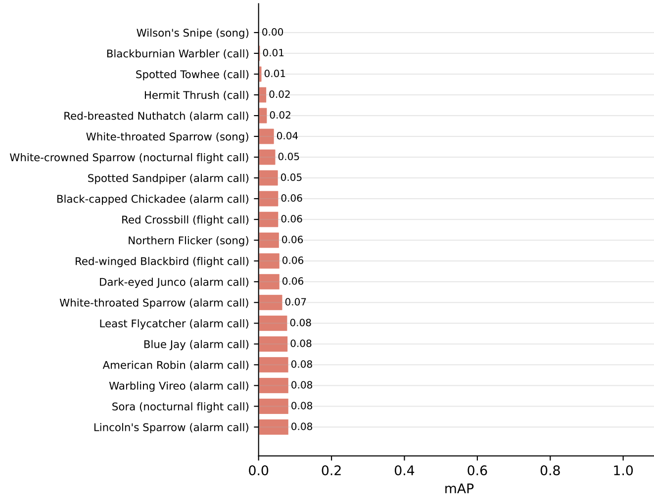
20 Hardest (lowest mAP)
